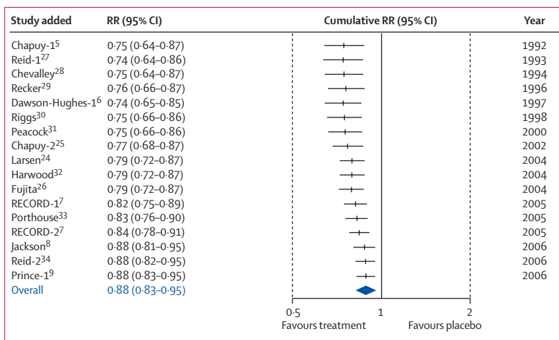
Figure 10: Cumulative meta-analysis
